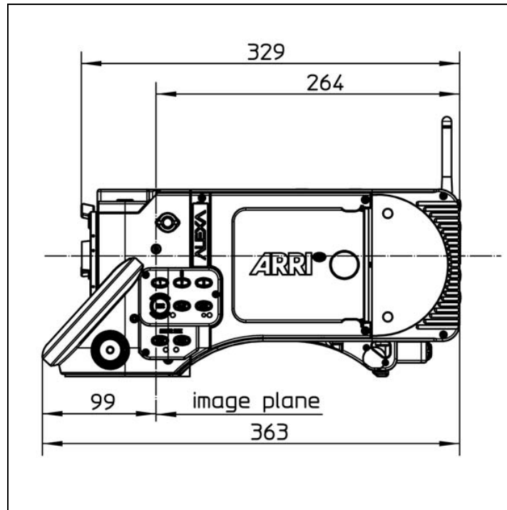
Figure 122: ALEXA Studio left
