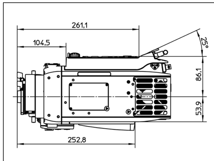
Figure 119: ALEXA Plus top
