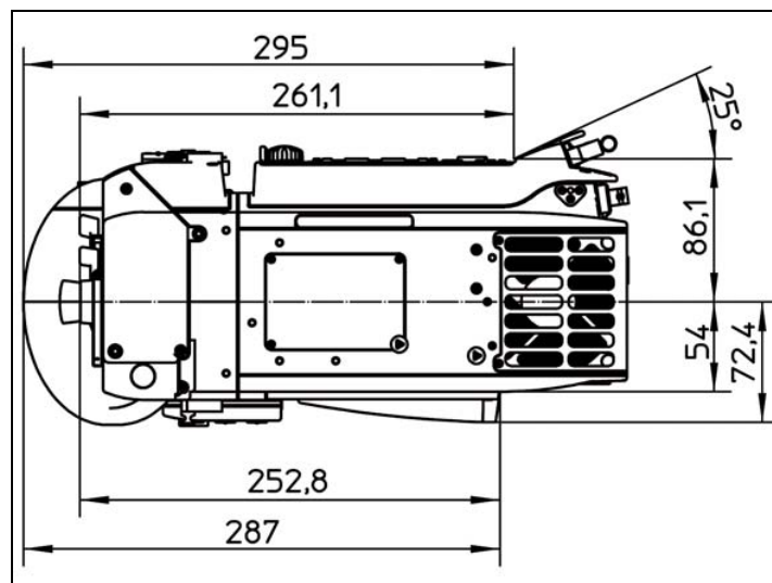
Figure 123: ALEXA Studio top
