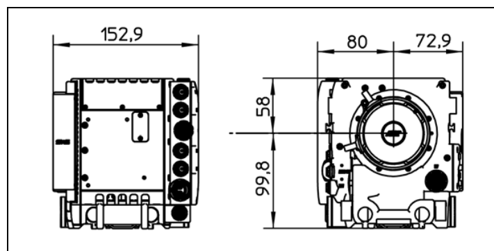
Figure 117: ALEXA front and back
