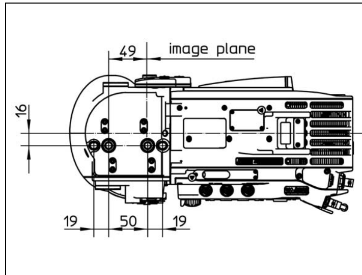
Figure 124: ALEXA Studio bottom
