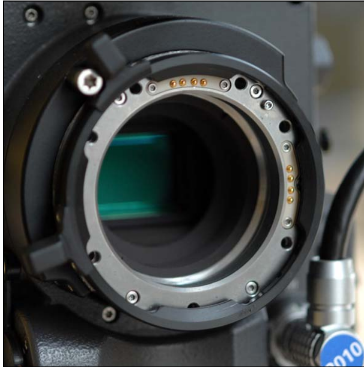
Figure 83: Lens adapter PL-Mount LA-PL-2 (with LDS)
