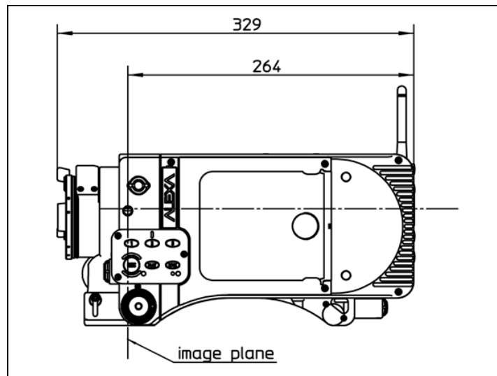
Figure 118: ALEXA Plus left
