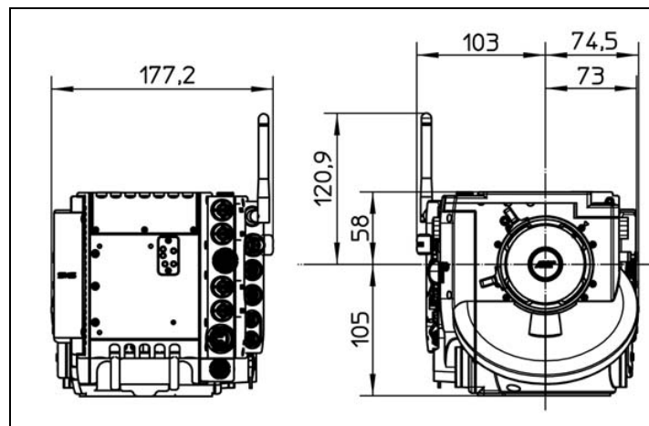
Figure 125: ALEXA Studio front and back
