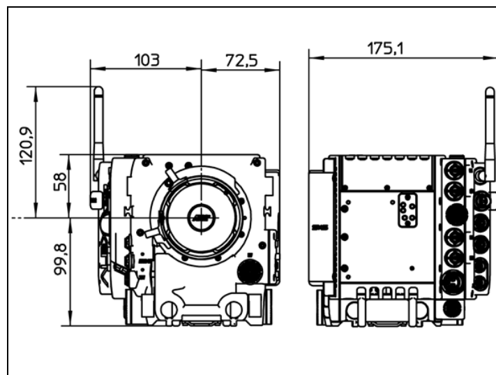
Figure 121: ALEXA Plus front and back
