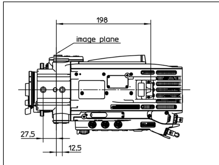
Figure 120: ALEXA Plus bottom
